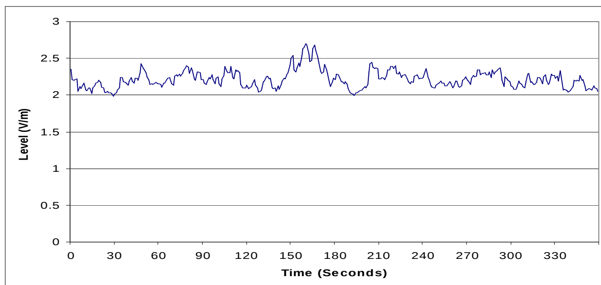
Electric field strengths recorded over 6 min period using 18 GHz probe at point of max NIR:
